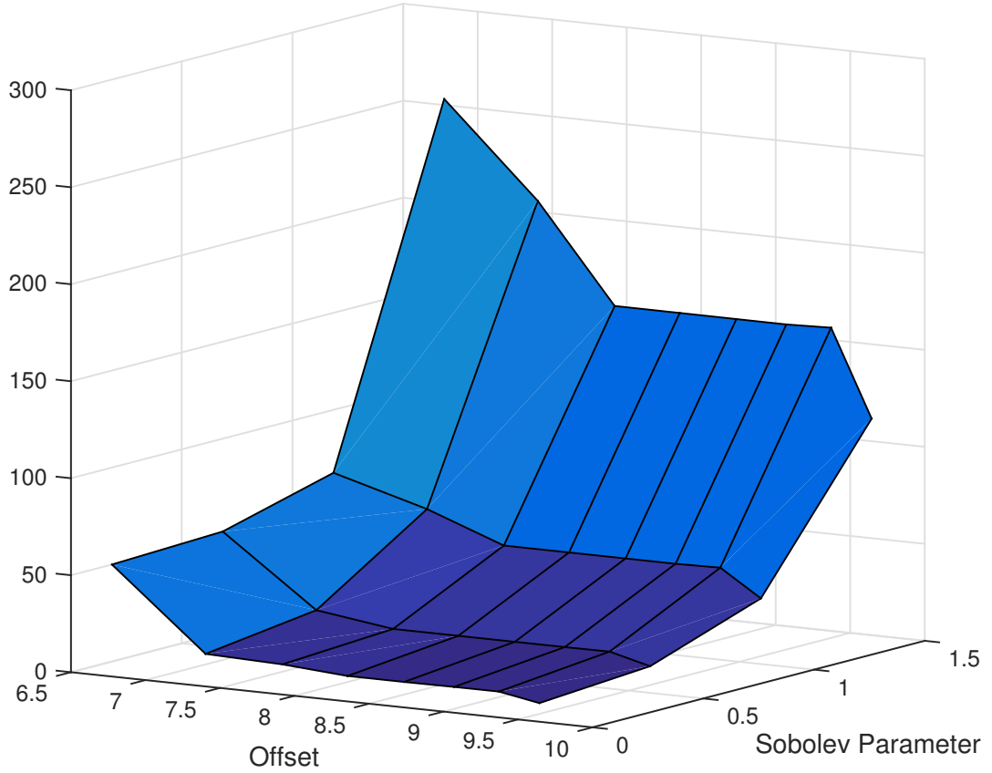
Figure 4: Largest singular value of \mathbf{W}\mathbf{T}_\Phi\mathbf{S}^{-1}\mathbf{T}_{\Phi_w}\mathbf{W}_w^{-1} with varying weights \mathbf{W}, \mathbf{W}_w and varying offset.
