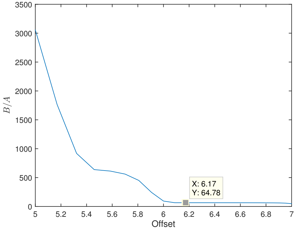
Figure 2: Quotient of the frame bounds for varying offset. One observes that for high offset the quotient becomes stable and explodes for decreasing offset.
